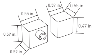
Silicone End Caps - Straight AL-02-71-9961-DS (1-pack) AL-02-71-9966-DS (10-pack)
