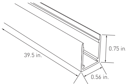
Aluminum Mounting Track AL-02-71-9923-AL (39.5 in.)
