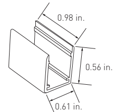
Aluminum Mounting Clip/Screws AL-02-71-9981 (1-pack) AL-02-71-9986 (10-pack)
