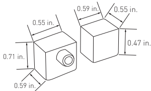
Silicone End Caps - Left/Right AL-02-71-9961 (1-pack) AL-02-71-9966 (10-pack)
