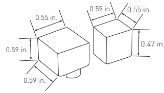
Silicone End Caps - Bottom AL-02-71-9961-BS (1-pack) AL-02-71-9966-BS (10-pack)
