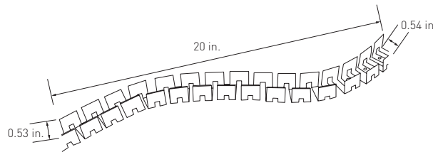
Flexible Mounting Track AL-02-71-9930 (20 in.)
