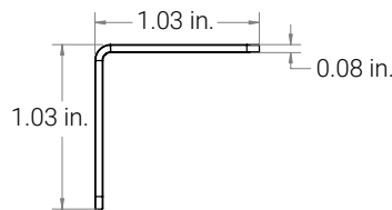
L Shaped 90 Degree Linker for Mitred Corners
