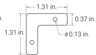
L Shaped 90 Degree Flat Plate Linker for Beveled Corners
