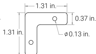
L Shaped 90 Degree Flat Plate Linker for Beveled Corners AL-50-81-9994-AL
