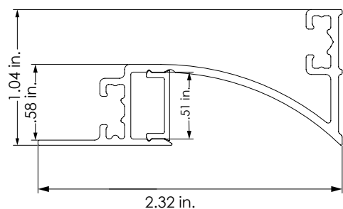
Ankr Perimeter 1 in.
