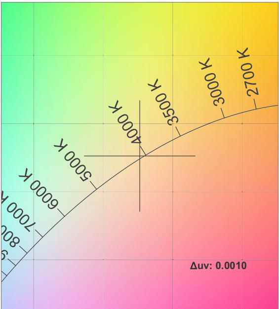
CRI: 92.7 (R1-R8)
