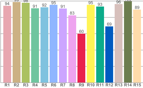
CRI: 92.7 (R1-R8)
