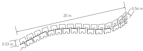
Flexible Mounting Track AL-01-71-9930 (20 in.)
