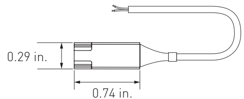
Tape Light Splice Connector
