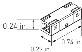
Tape-to-Tape Connector
