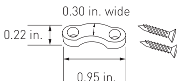
Wire Harness Holds wire in place securely AL-01-99-9901-10 (10-pack)
